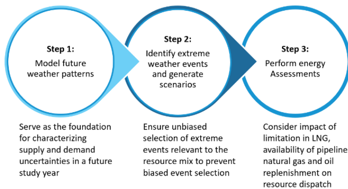
Figure 2.5: PEAT Framework
